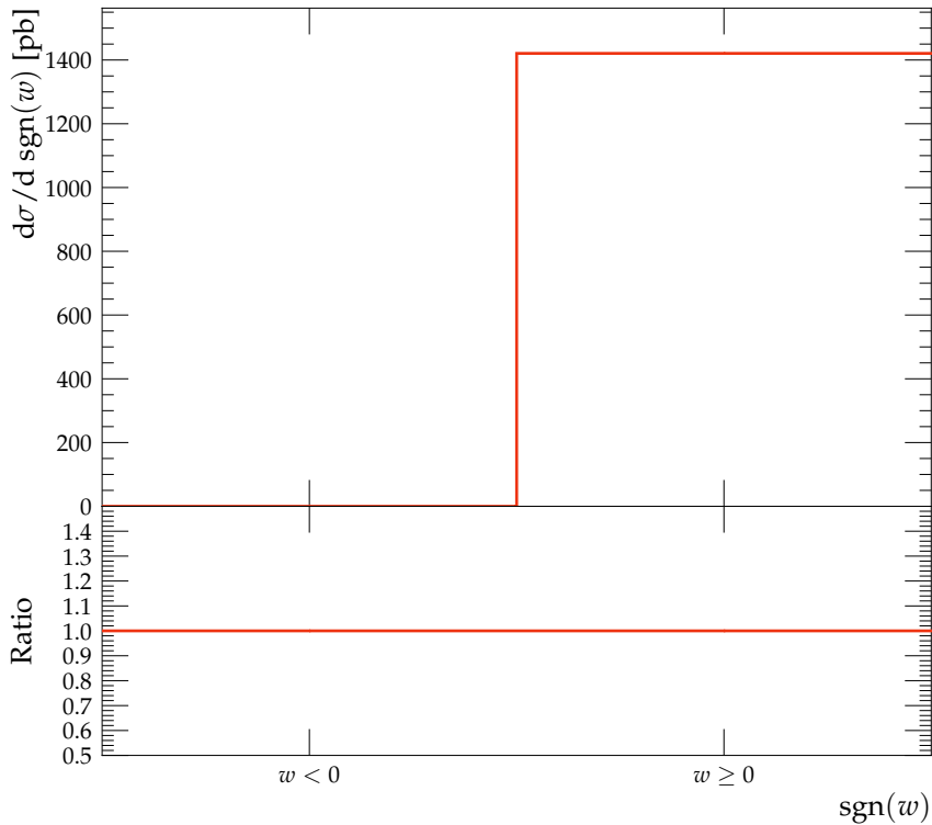
Fraction of positive and negative weighted events
